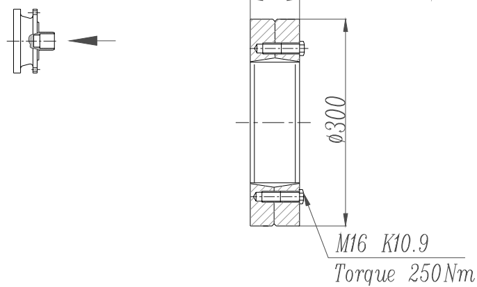
Shrink disc
