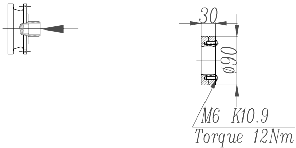
Shrink disc
