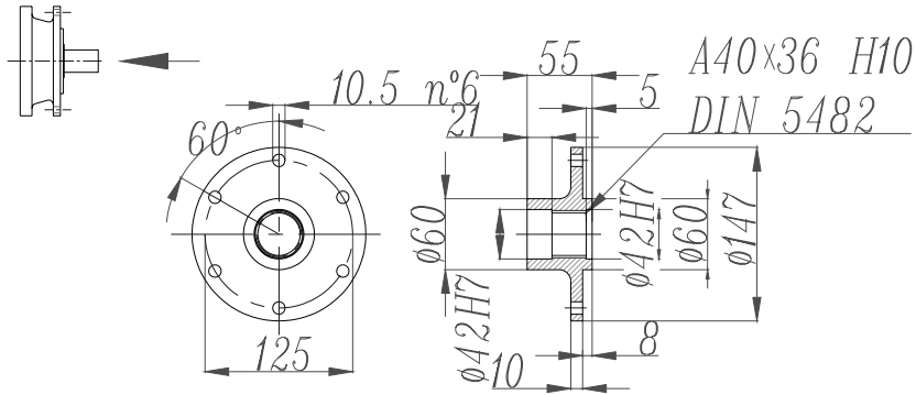
Drive intake flange
